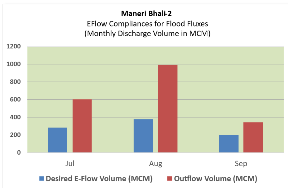
Figure 3: Graphs showing status of implementation of E-Flow at Maneri Bhali- II
