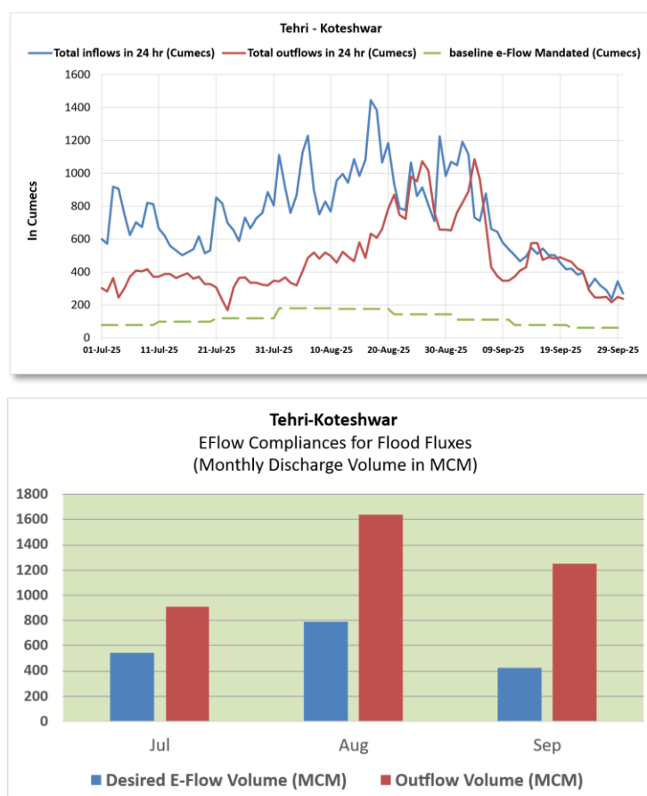
Figure 4: Graphs showing status of implementation of E-Flow at Tehri – Koteswar
