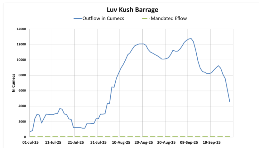
Figure 12: Graph showing status of implementation of E-Flow at Lav Kush Barrage Project.
