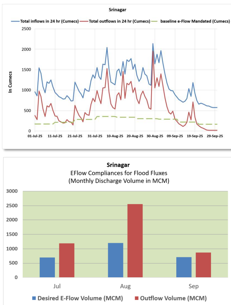
Figure 7: Graphs showing status of implementation of E-Flow at Srinagar HEP
