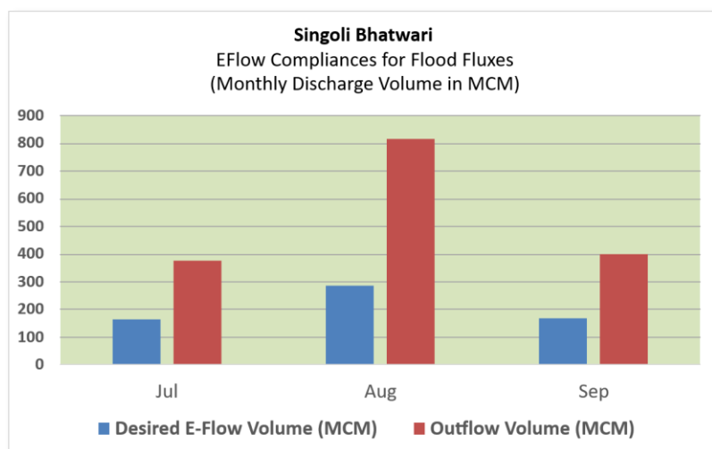
Figure 6: Graphs showing status of implementation of E-Flow at Singoli Bhatwari HEP
