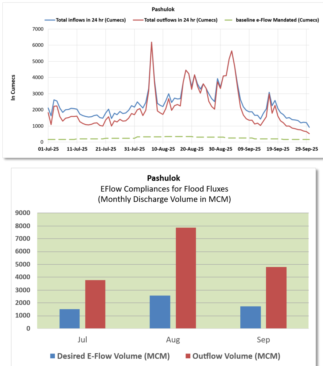
Figure 8: Graphs showing status of implementation of E-Flow at Pashulok Barrage
