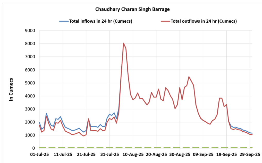
Figure 10: Graph showing status of implementation of E-Flow at Chaudhary Charan Singh Barrage
