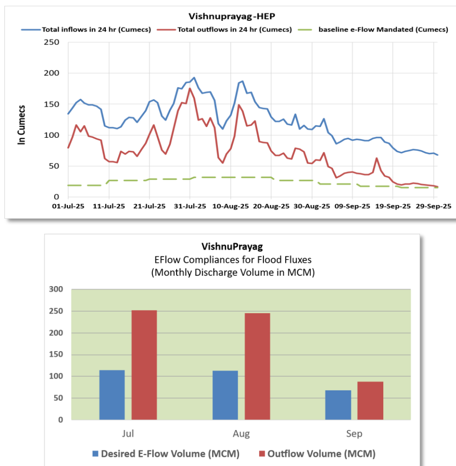
Figure 5: Graphs showing status of implementation of E-Flow at Vishnuprayag HEP
